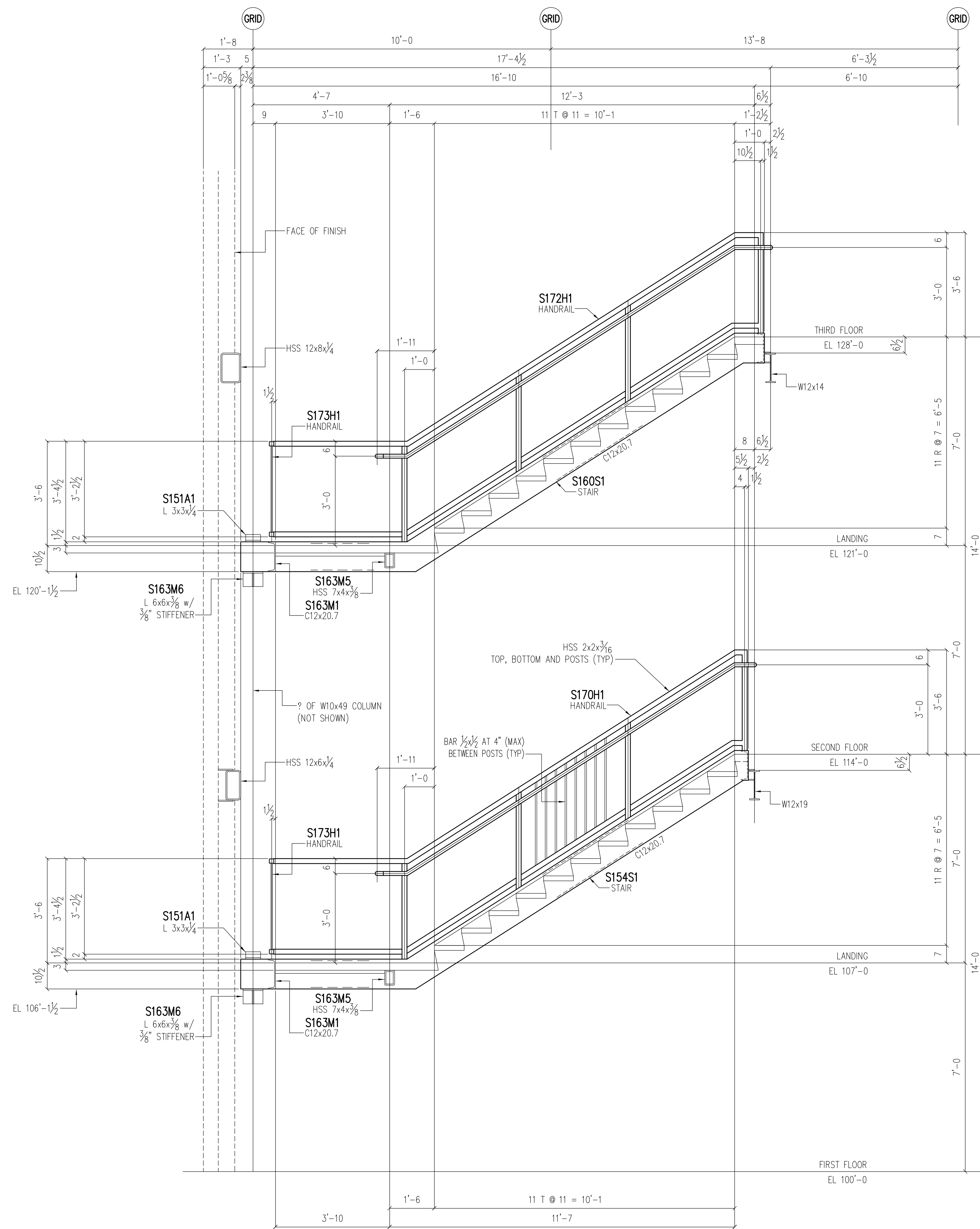
SECTION A-A/SE113 (LOOKING NORTH) [ SE110, SE111 ]
