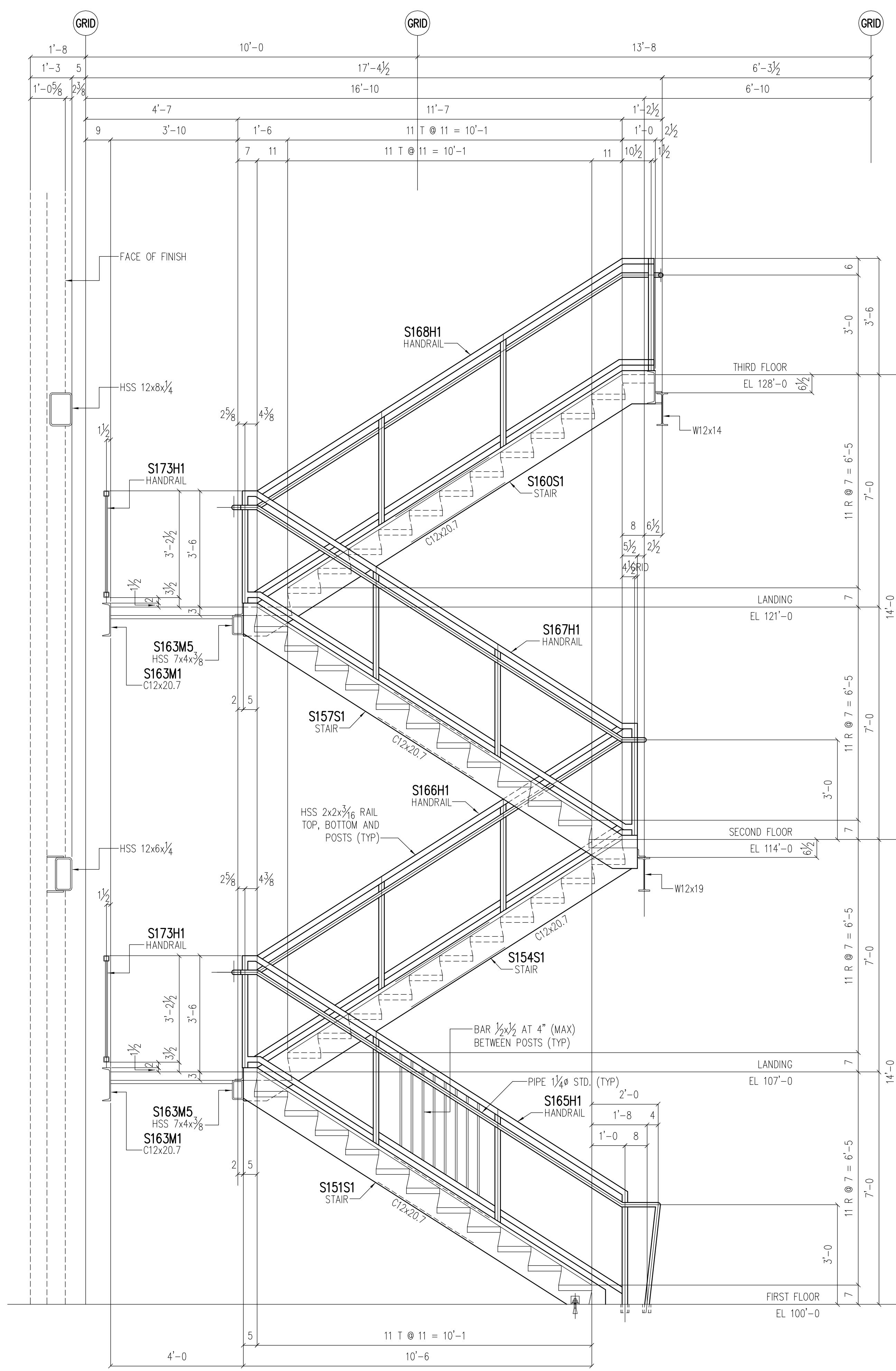
SECTION A-A/E112 (LOOKING NORTH) [ SE110, SE111 ]
