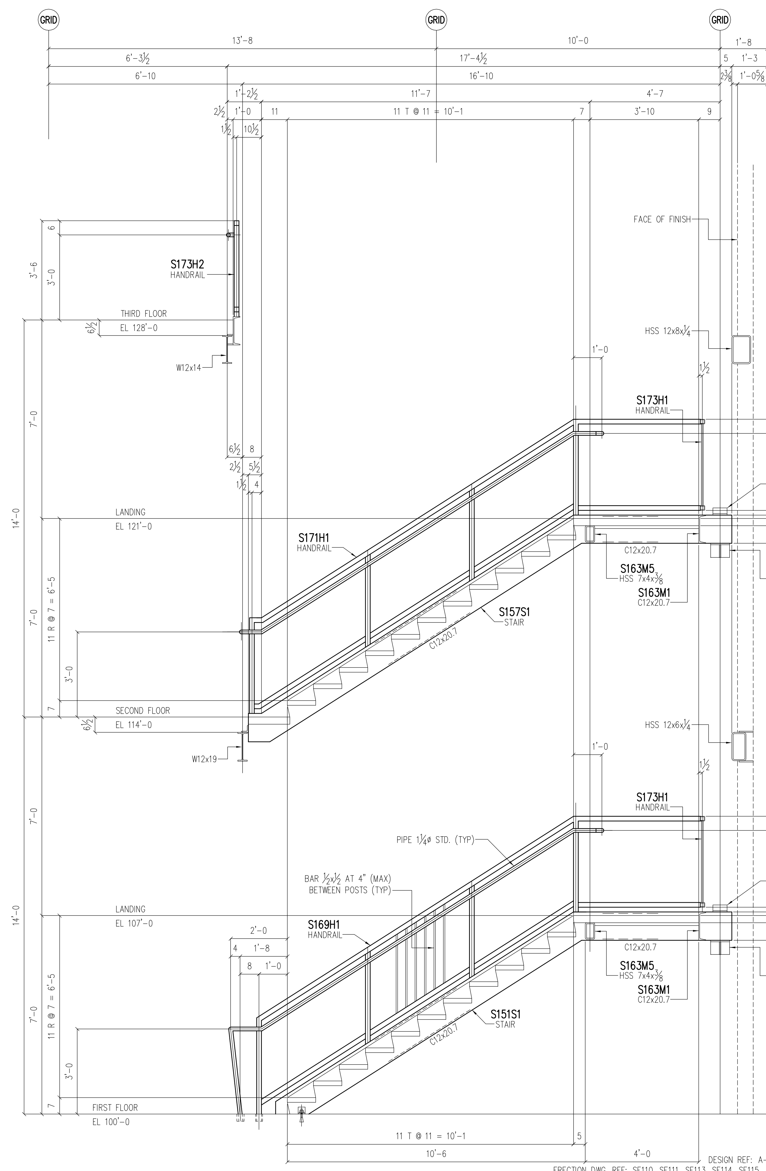
SECTION B-B/E112 (LOOKING SOUTH) [ SE110, SE111 ]
