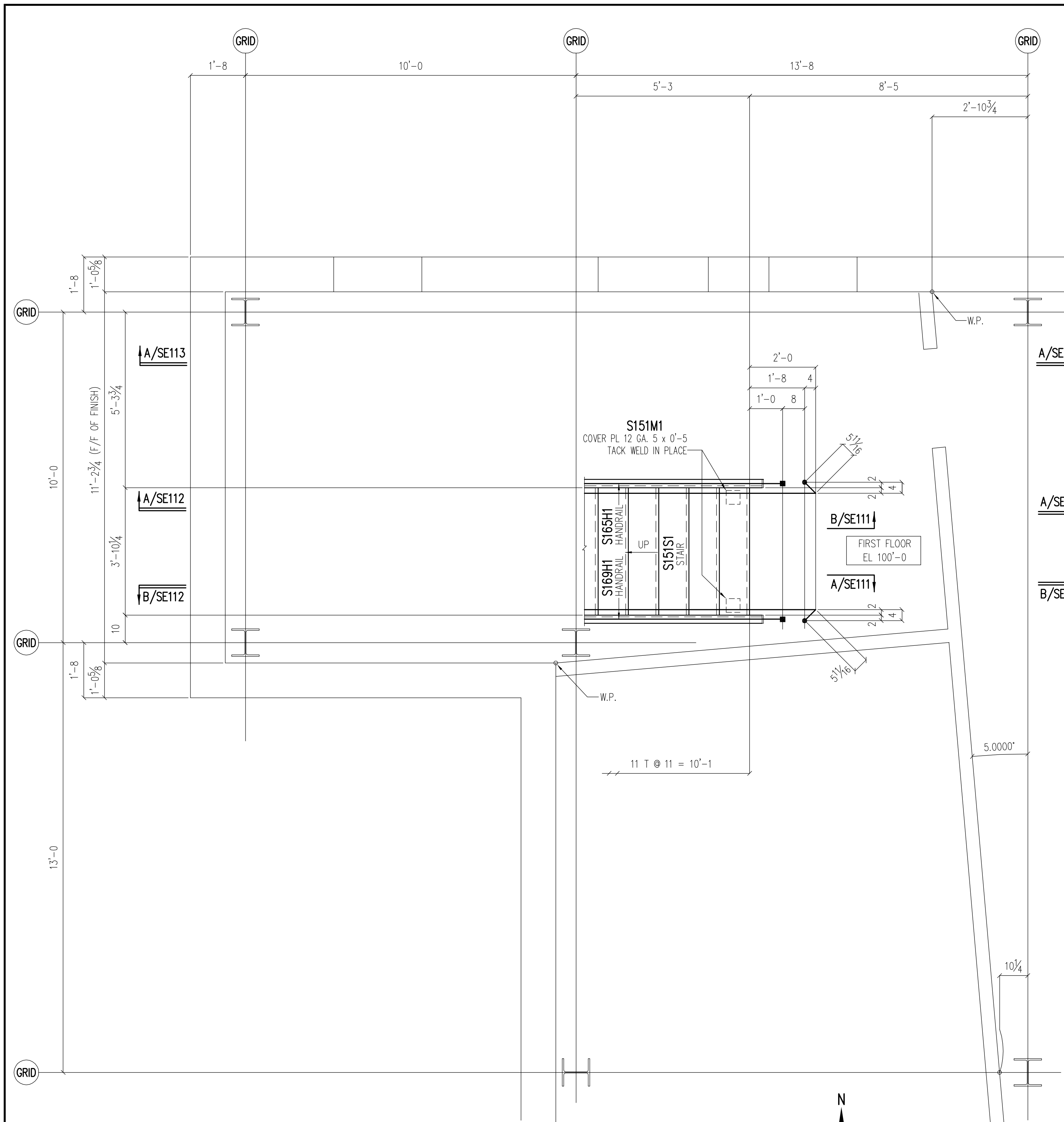
PLAN AT STAIR NO. C02 - FIRST FLOOR
