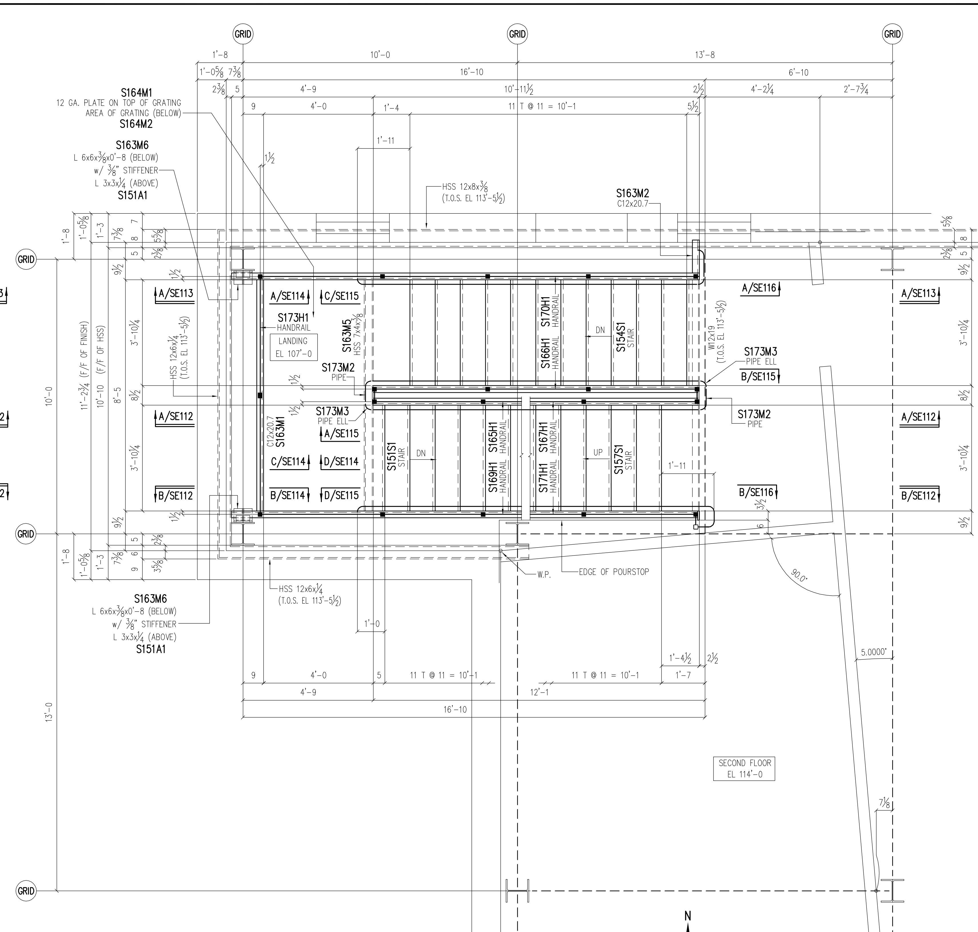
PLAN AT STAIR NO. C02 - SECOND FLOOR
