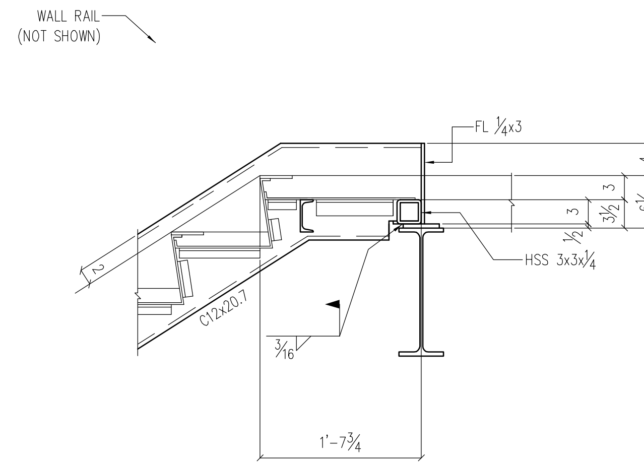
SECTION F/SE108 [ SE102 ]
