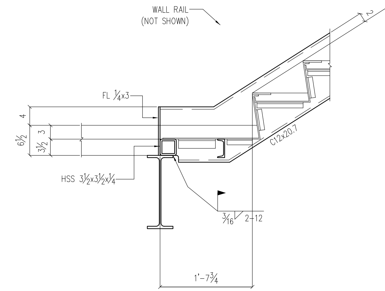
SECTION G/SE108 [ SE102 ]
