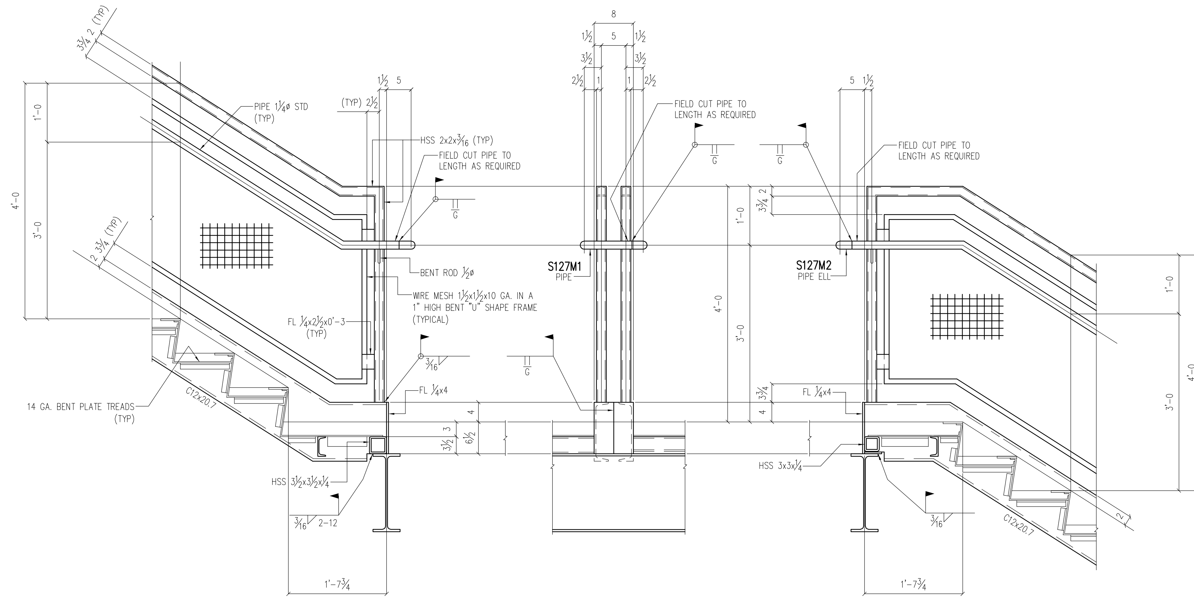
SECTION A/SE108 [ E102 ]
