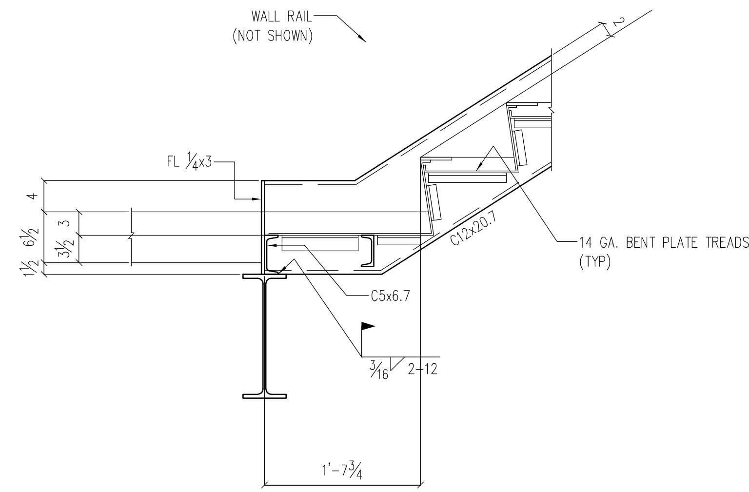
SECTION C/SE108 [ SE101 ]
