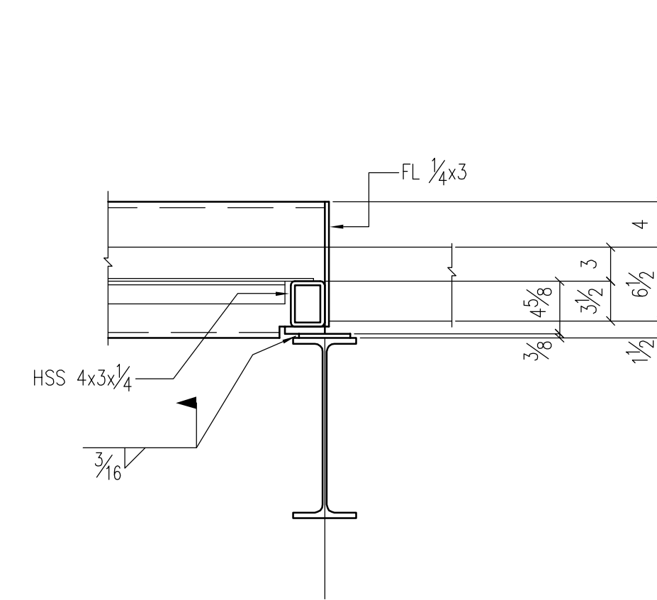
SECTION D/SE108 [ SE101 ]
