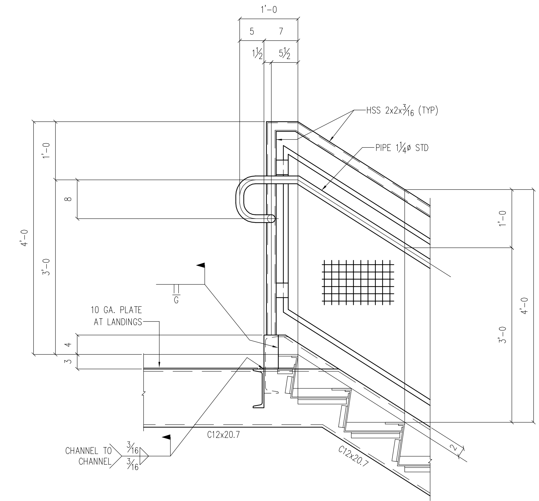
SECTION B/SE108 [ SE102 ]
