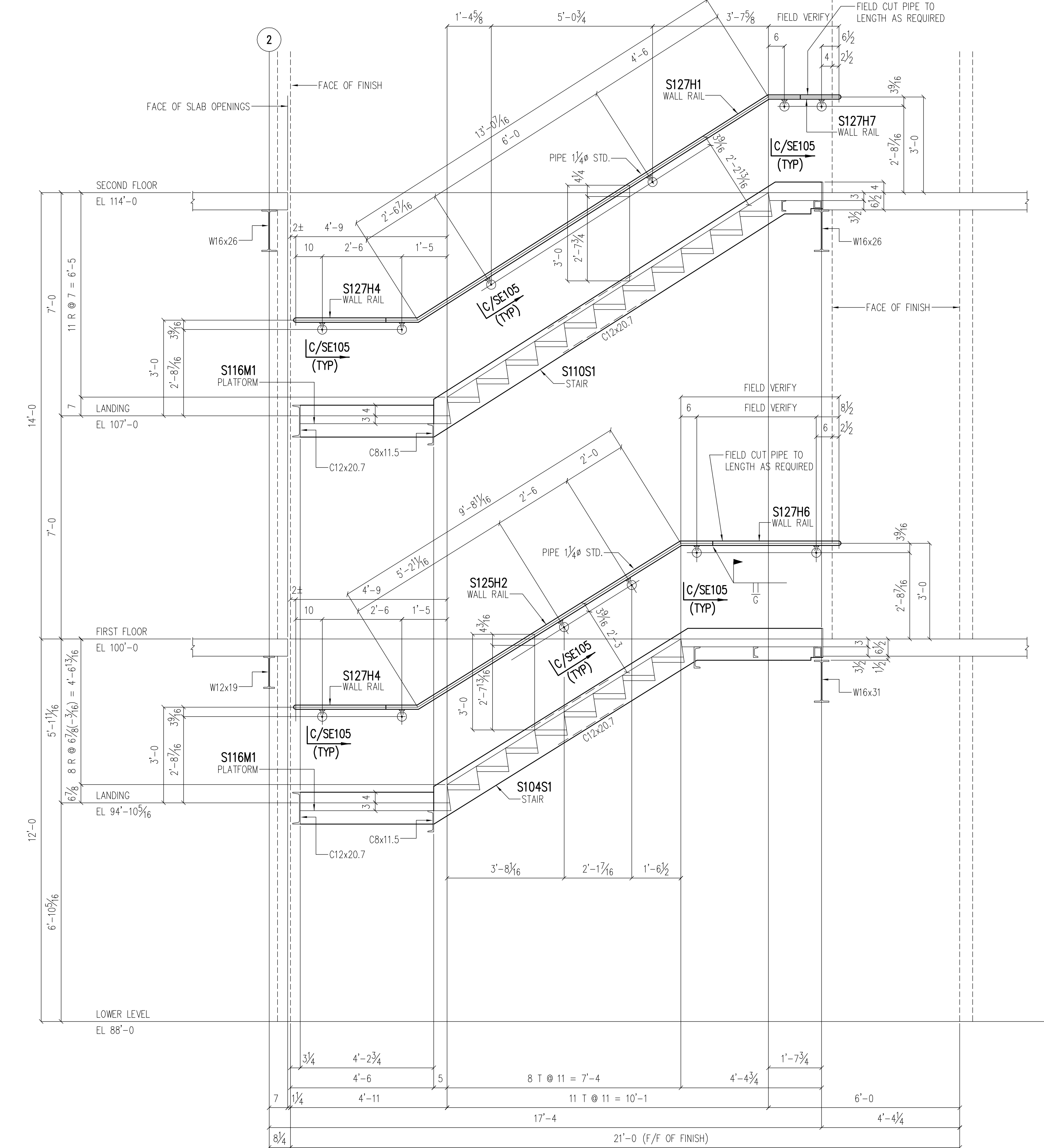
SECTION B-B/SE105 (STAIR NO. 2 - LOOKING NORTH) [ SE101, SE102 ]
