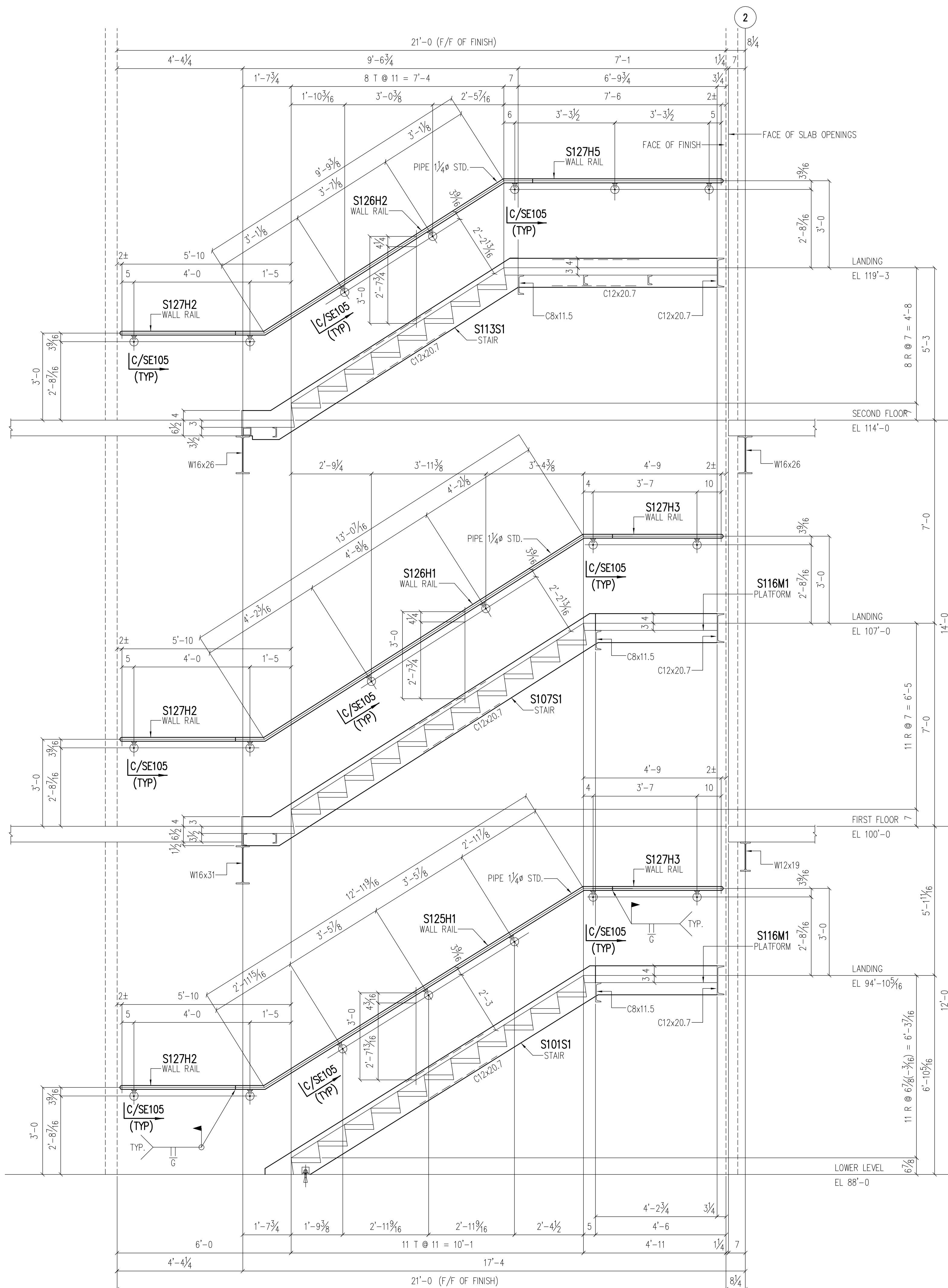
SECTION A-A/SE105 (STAIR NO. 2 - LOOKING SOUTH) [ SE101, SE102 ]
