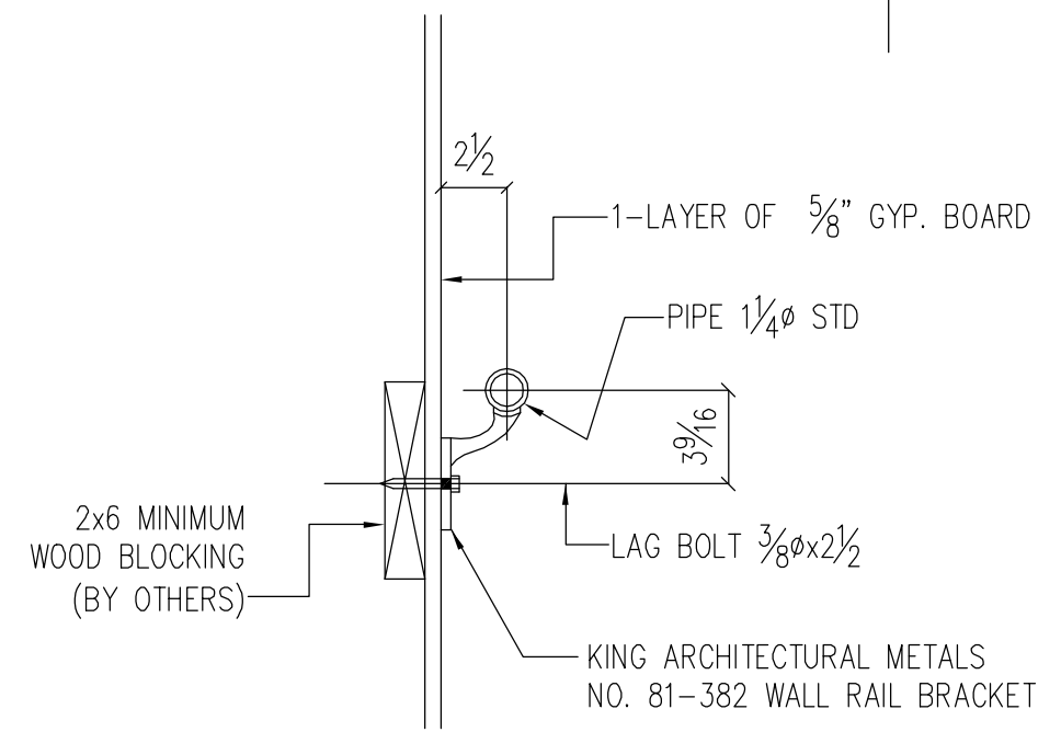
SECTION C-C/SE105 [ SE105 ]
