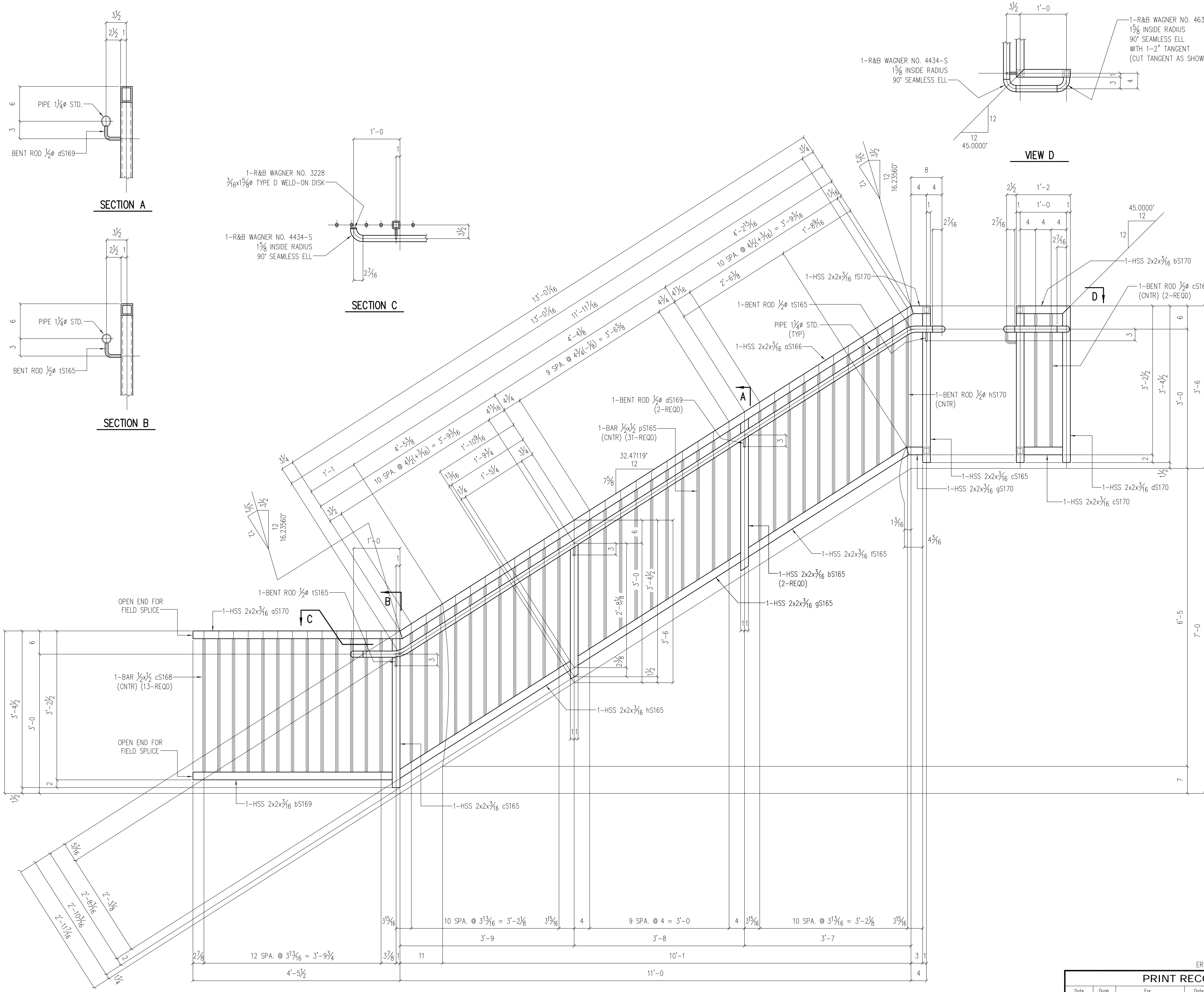
ONE HANDRAIL S170H1
