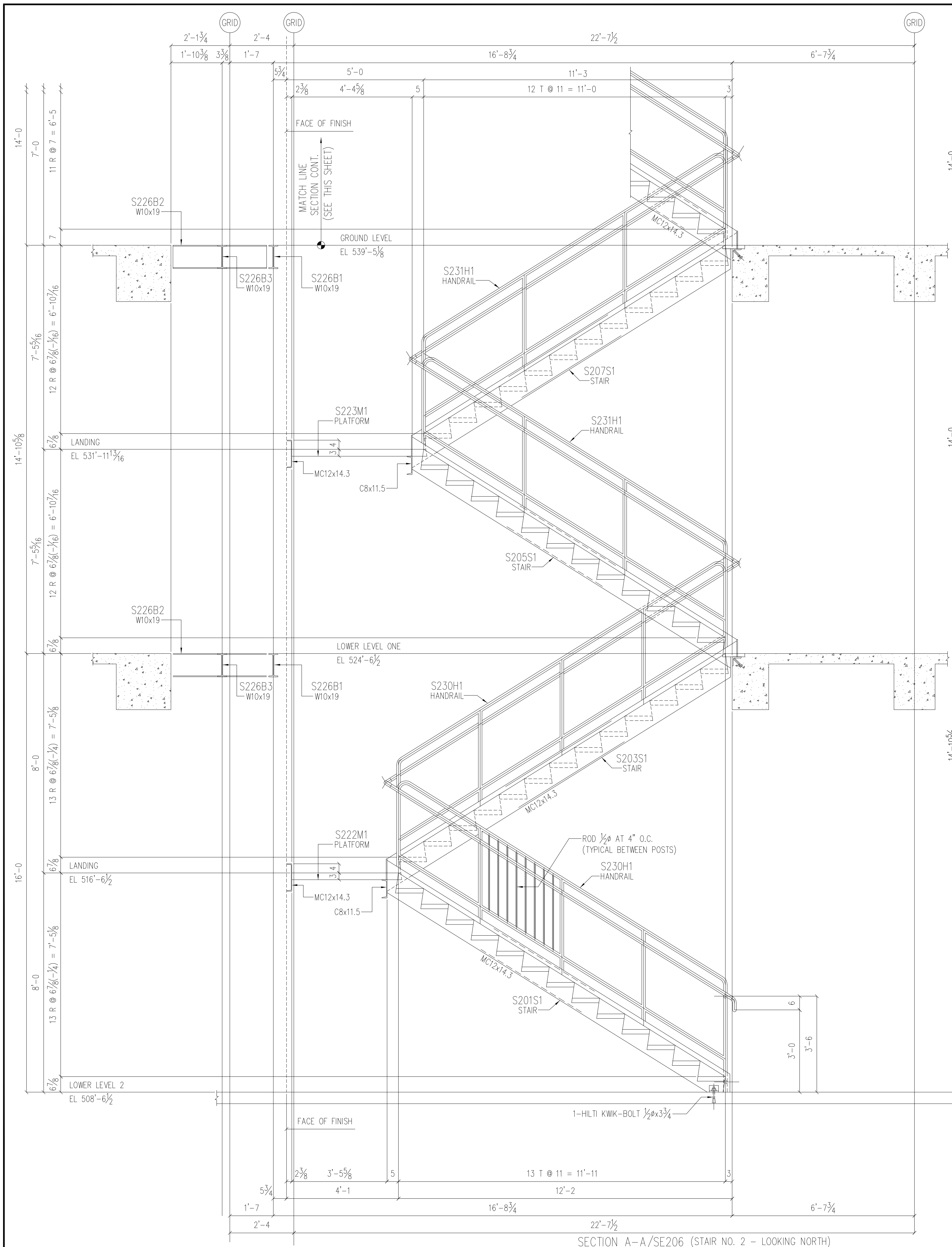
SECTION A-A/SE206 (STAIR NO. 2 - LOOKING NORTH) [ SE200, SE201, SE202, SE203, SE204, SE205 ]
