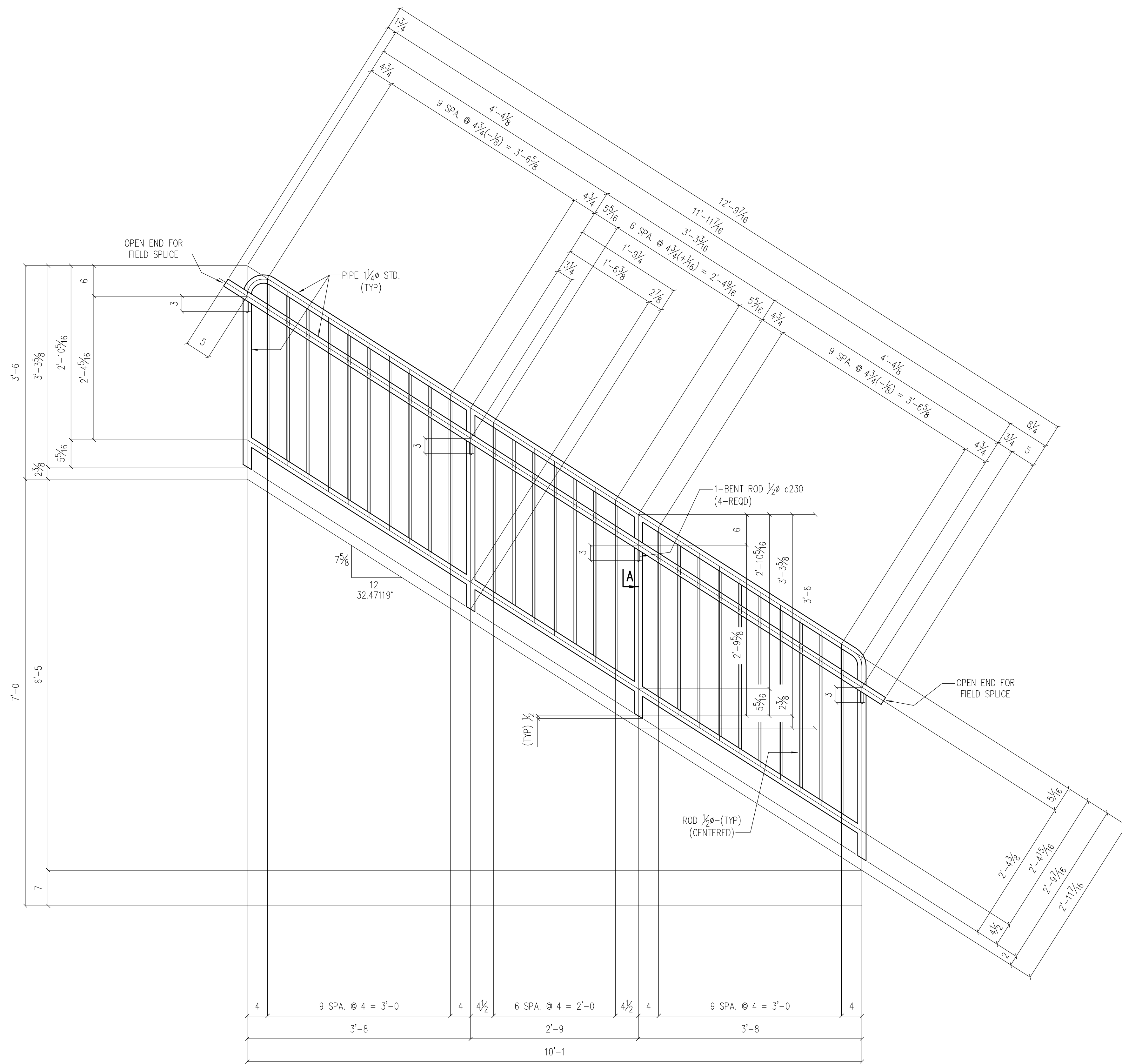
4 HANDRAILS S232H1
